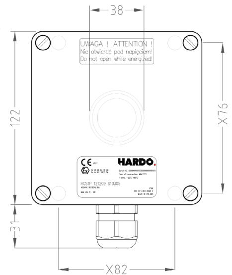
x - mounting dimensions
